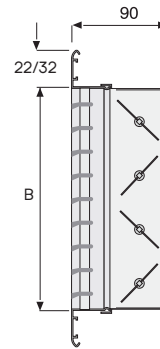
Tek Sıra Zıt Damperli Single Row With Damper
